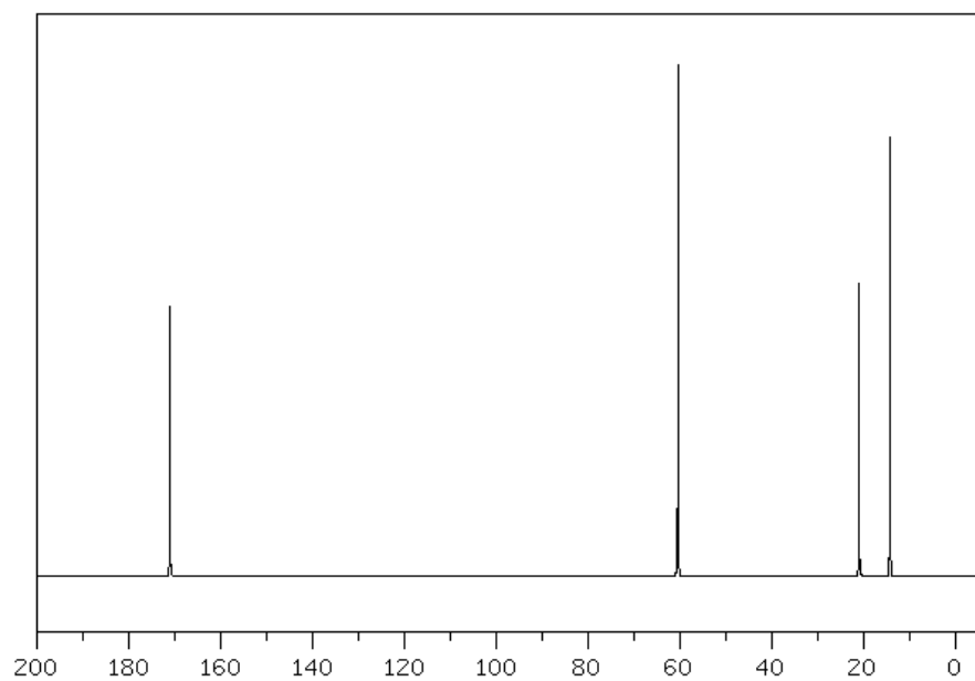
B: 2-methylpropanoic acid
