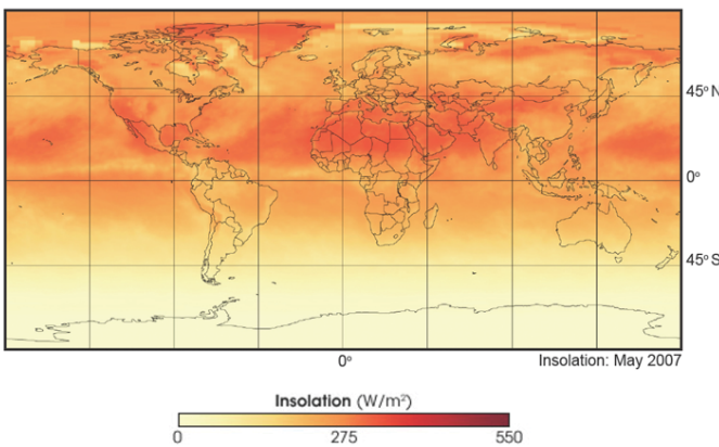
May Incoming Solar Radiation
