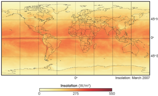
March Incoming Solar Radiation
