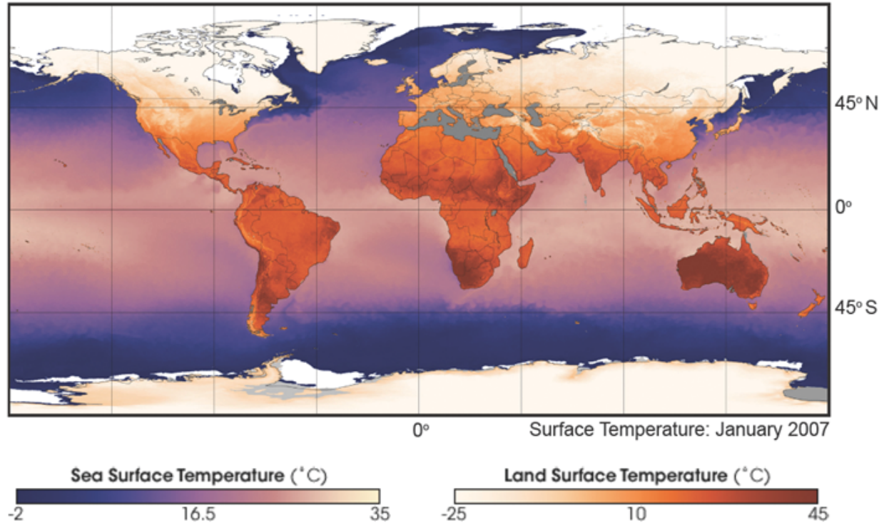
Figure EA-I-13: Global Surface Air Temperature in January and July, 1988.
