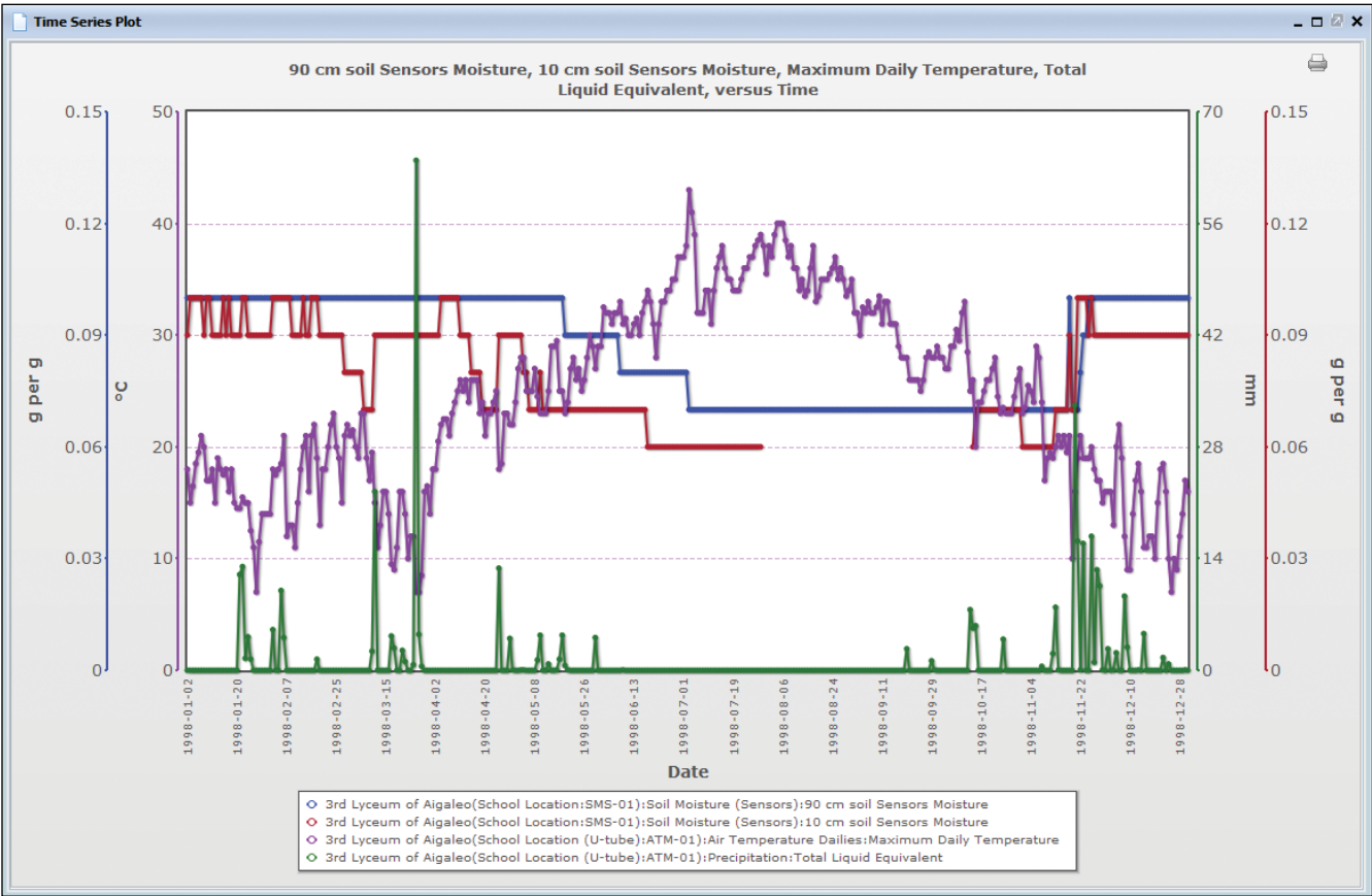
Figure EA-I-21: Maximum air temperature (purple), precipitation (green), and soil moisture at 10 (red) and 90 (blue) cm at 3rd Lyceum of Aigaleo in Athens, Greece, January 1, 1998 to December 31, 1998.
