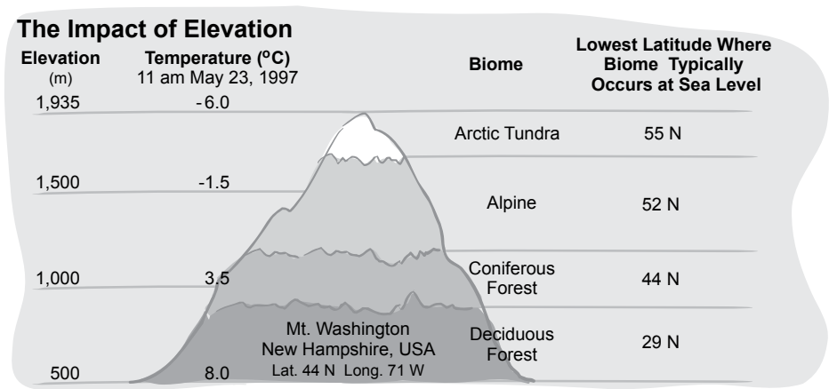
Figure EA-I-11: Impact of Elevation on Climate Zone
