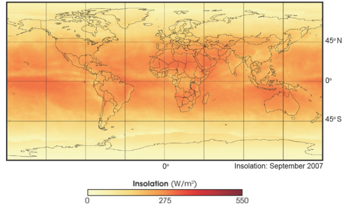
September Incoming Solar Radiation
