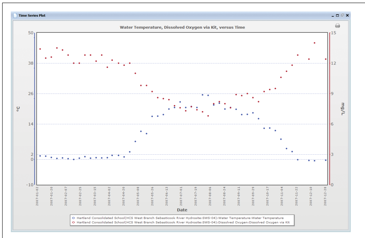
Figure EA-I-19: Surface water temperature and dissolved \text{O}_2 at Hartland Consolidated School in 2007
