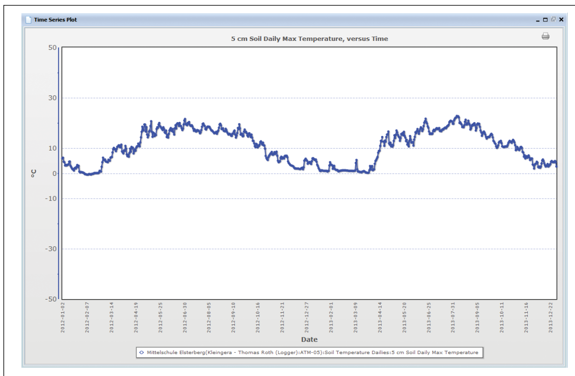
Figure EA-I-20: Seasonal cycle of the 5 cm soil temperature at Mittelschule Elsterberg in Elsterberg, Germany from January 1, 2012 to December 31, 2013.
