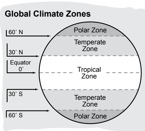
Figure EA-I-8: Approximate Global Climate Zones
