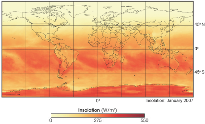
January Incoming Solar Radiation
