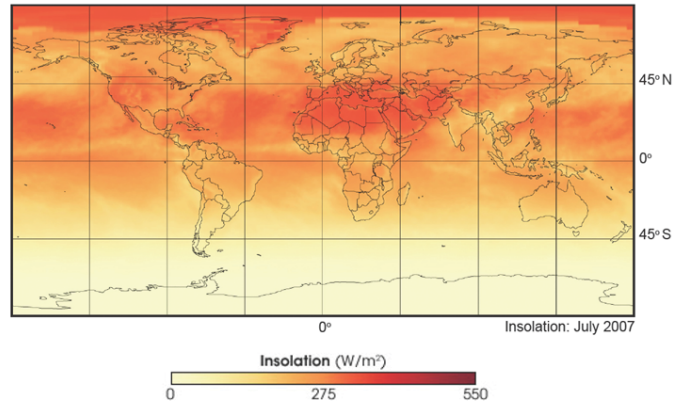
July Incoming Solar Radiation
