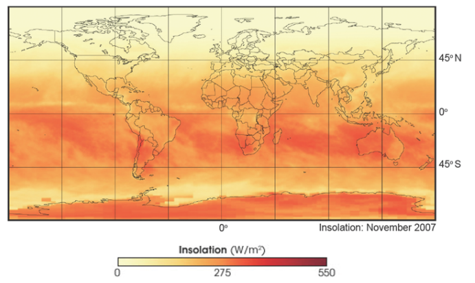
November Incoming Solar Radiation
